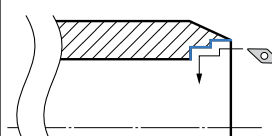
C45, Statorwelle
